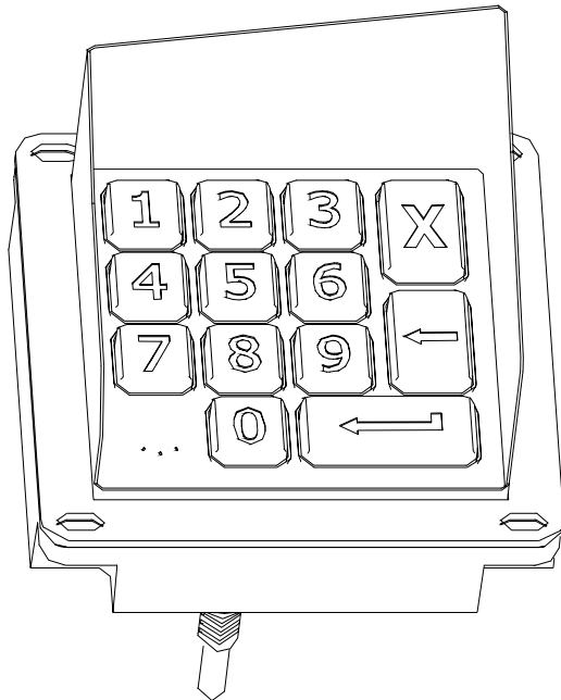
Figure 3B: Privacy shield relative to Keys & faceplate, SmartPIN without LCD
